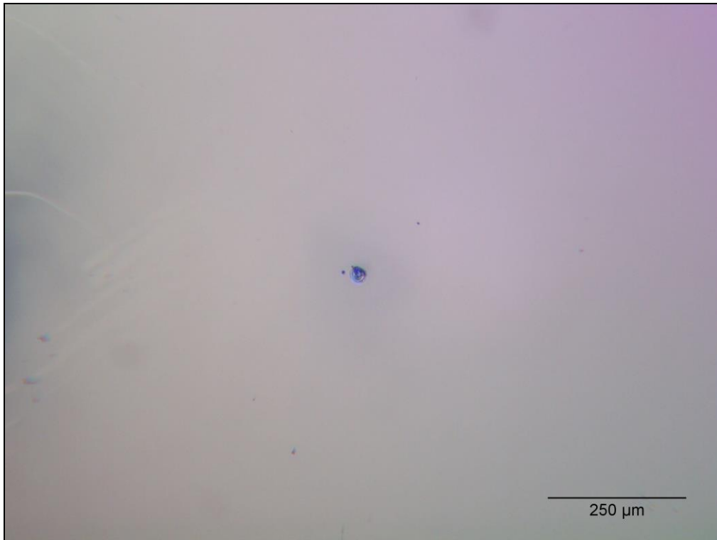
Fig. 5. Typical rear surface damage morphology (Energy density 30.42 J/cm 2 , damage after 11 pulses)
