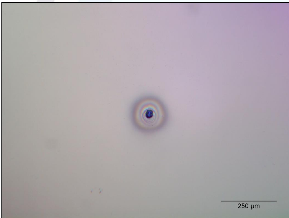
Fig. 4. Typical front surface damage morphology (Energy density 15.06 J/cm 2 , damage after 602 pulses)
