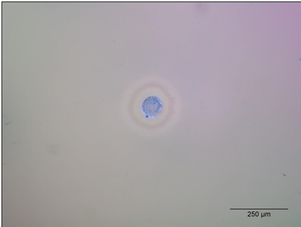
Fig. 3. Typical front surface damage morphology (Energy density 30.42 J/cm 2 , damage after 11 pulses)
