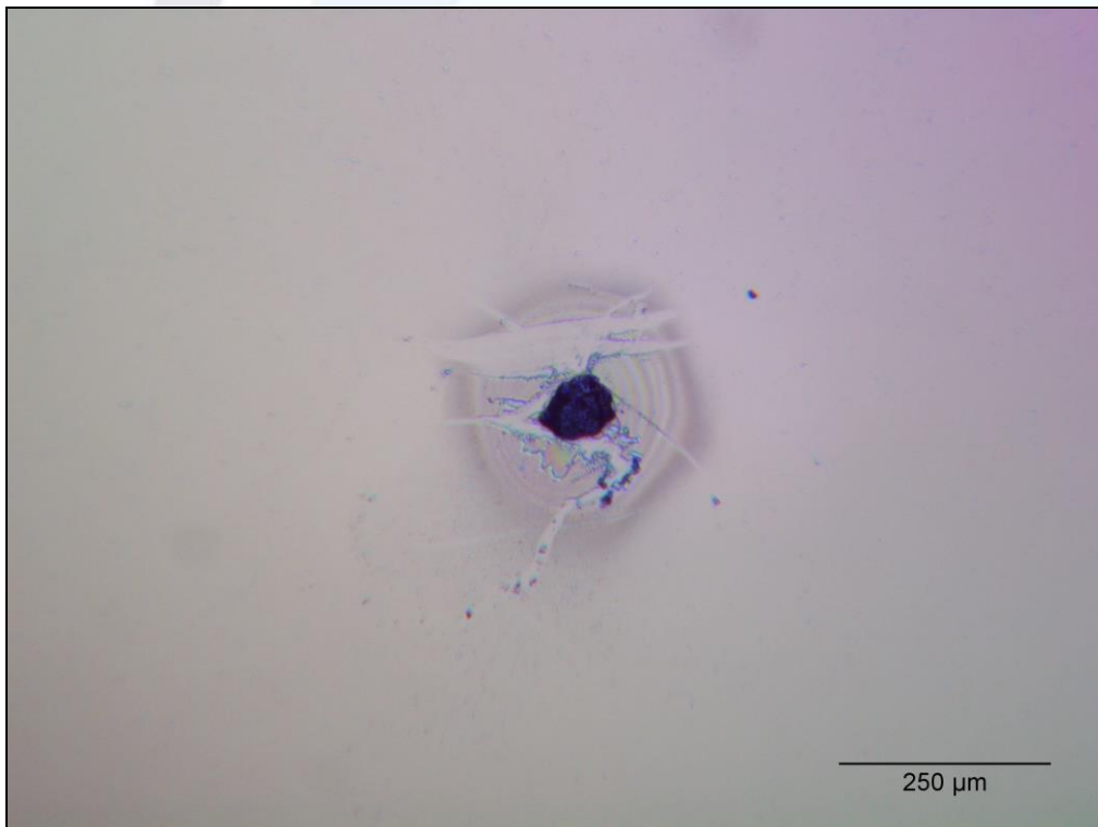
Fig. 6. Typical rear surface damage morphology (Energy density 12.40 J/cm 2 , damage after 1000 pulses)
